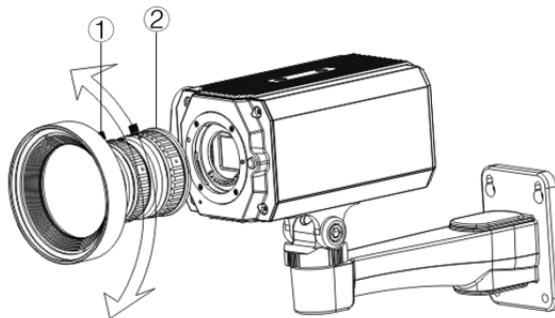
Figure 8-3 Lens installation (2)
