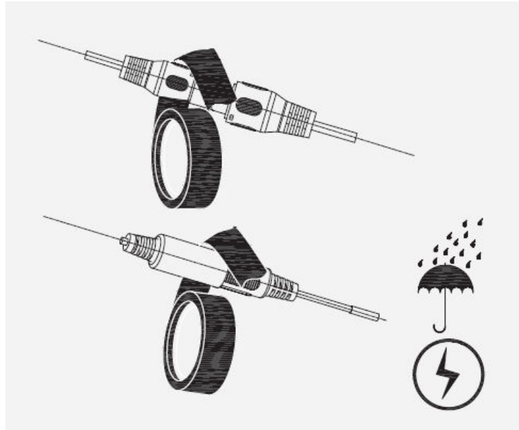
Figure 10-4 Waterproof measures
